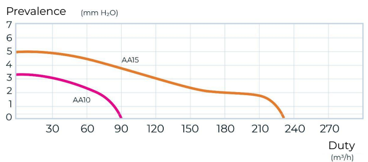
Flow rate curve
